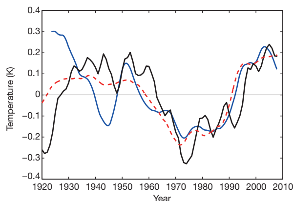
Figure 3 | Sea-level circulation index, the NAO and the AMO on multi-decadal timescales. Shown are the accumulated sea-level index (blue), which is representative of subpolar heat content evolution, the accumulated NAO (red, dashed) and the AMO (black). The heat content proxy and the accumulated NAO have been normalized. All timeseries have been 7-year low-pass filtered. The accumulated sea-level index and accumulated NAO have been detrended.
